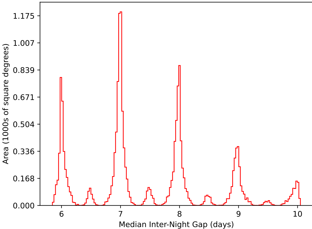
baseline_v2.0_10yrs WFD i band: Median Inter-Night Gap
