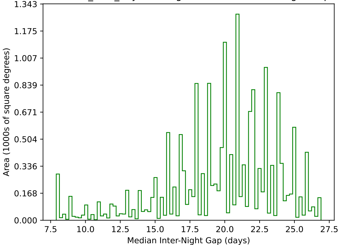
baseline_v2.0_10yrs WFD g band: Median Inter-Night Gap
