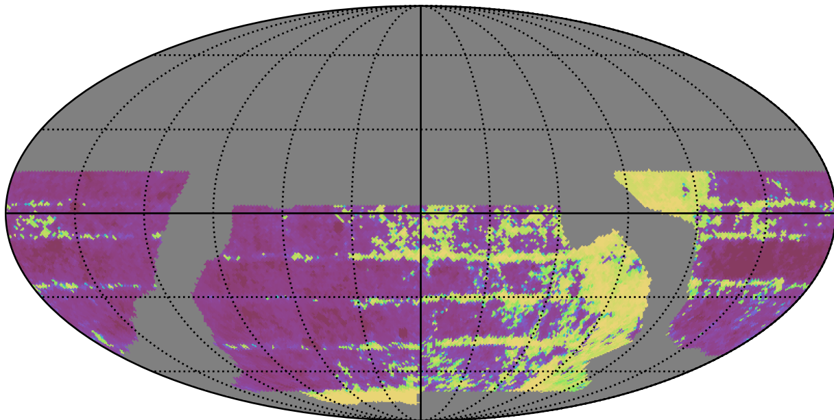
baseline_v2.0_10yrs WFD all bands: Median Inter-Night Gap
