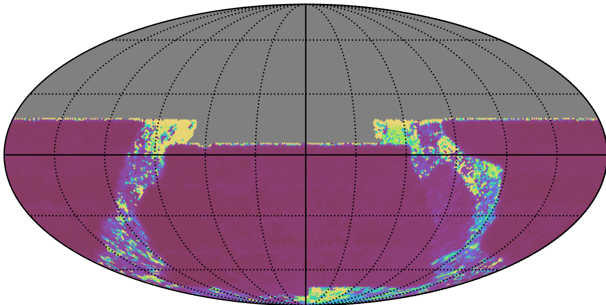
baseline_v2.0_10yrs All sky y band: Median Inter-Night Gap
