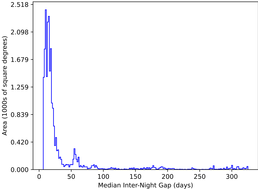
baseline_v2.0_10yrs All sky y band: Median Inter-Night Gap
