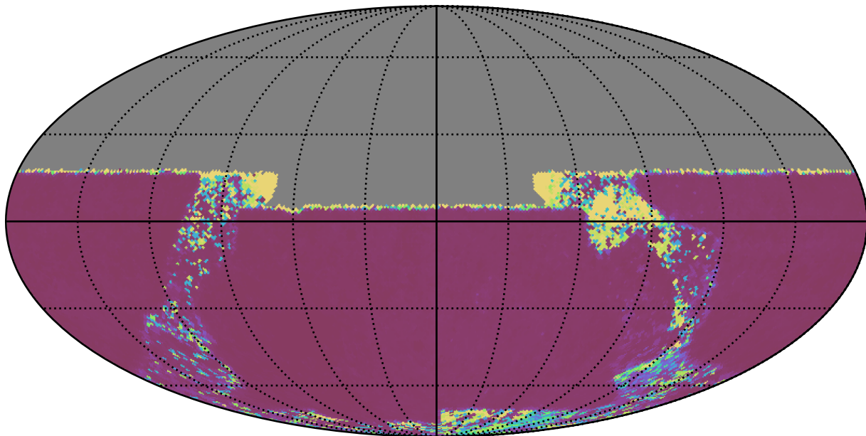
baseline_v2.0_10yrs All sky u band: Median Inter-Night Gap
