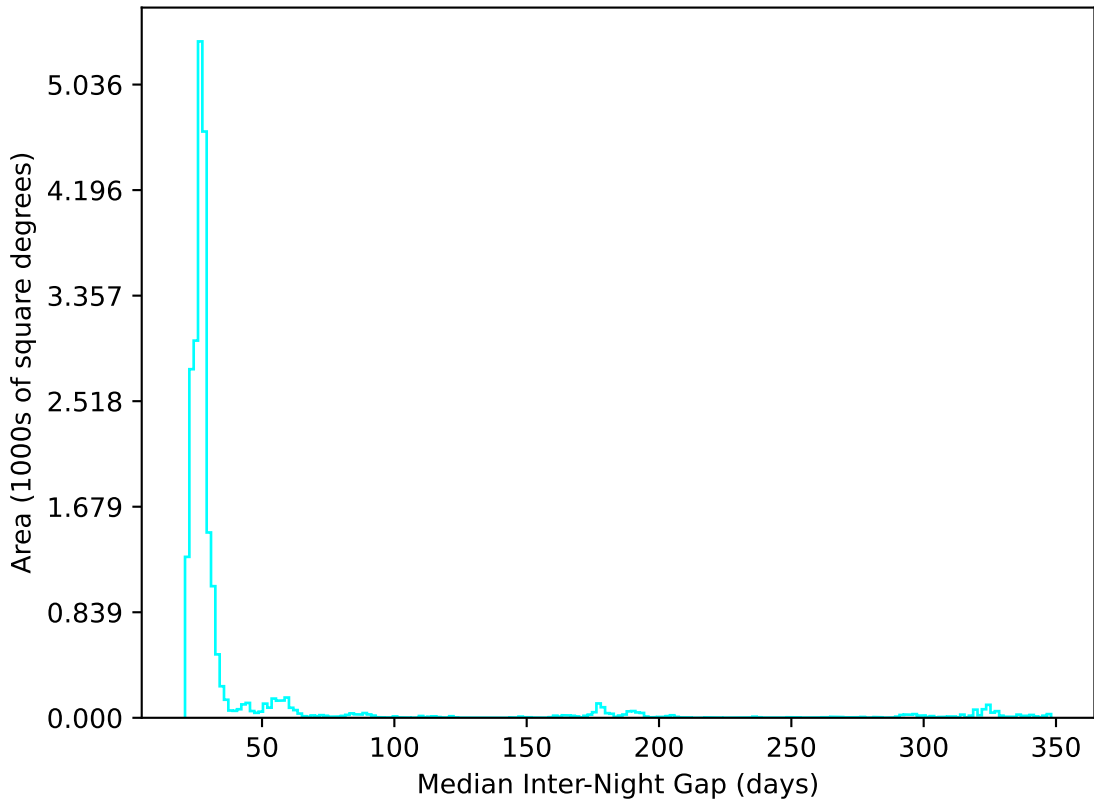
baseline_v2.0_10yrs All sky u band: Median Inter-Night Gap
