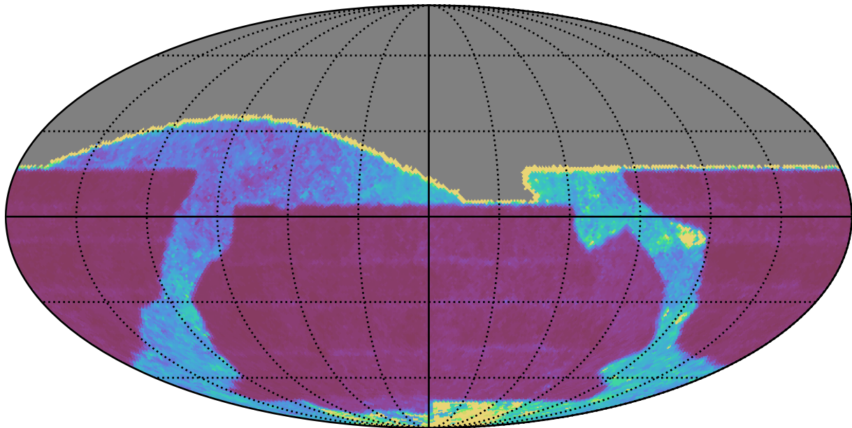
baseline_v2.0_10yrs All sky r band: Median Inter-Night Gap
