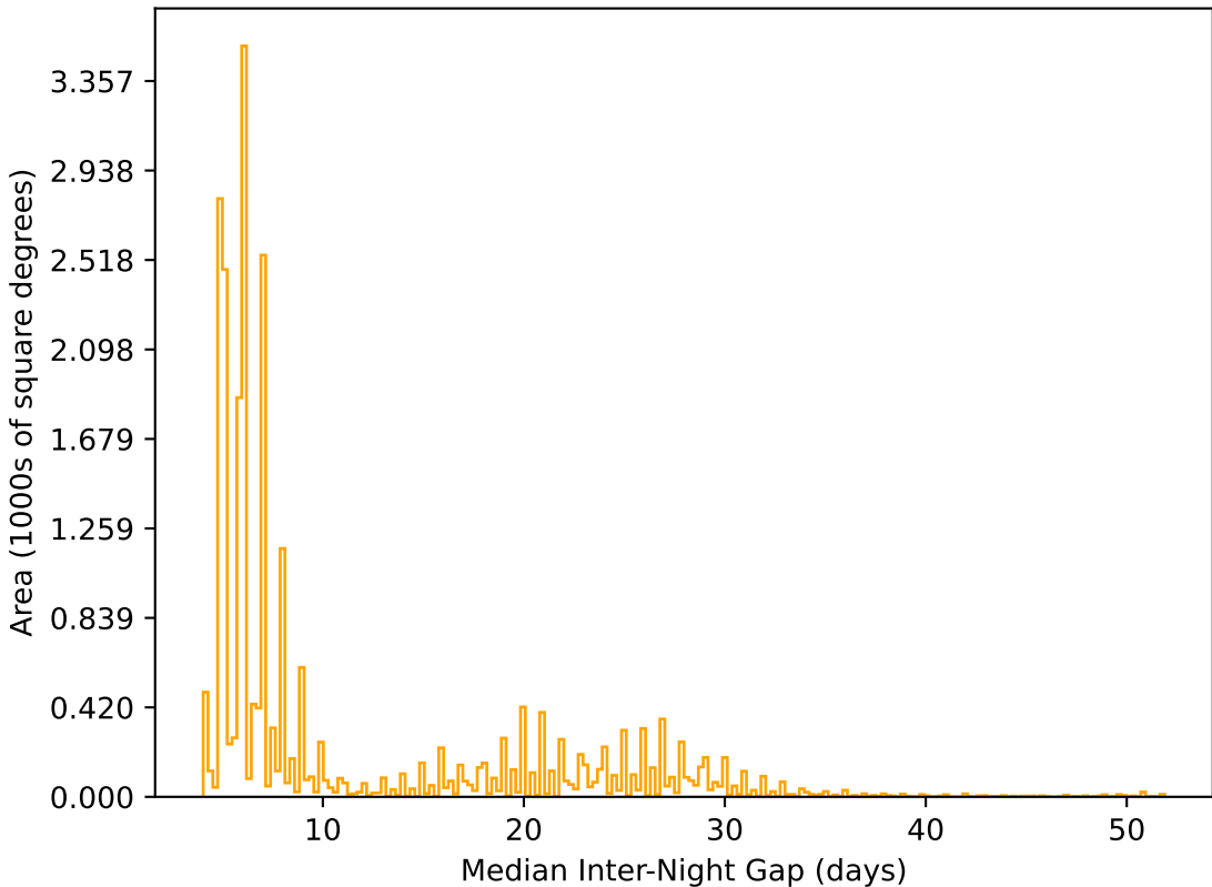
baseline_v2.0_10yrs All sky r band: Median Inter-Night Gap
