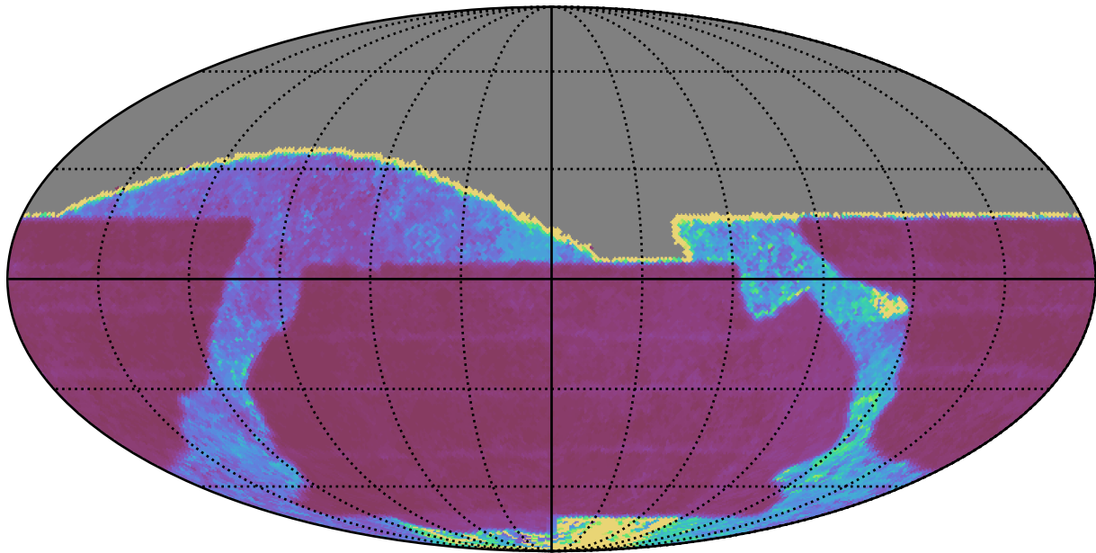
baseline_v2.0_10yrs All sky i band: Median Inter-Night Gap
