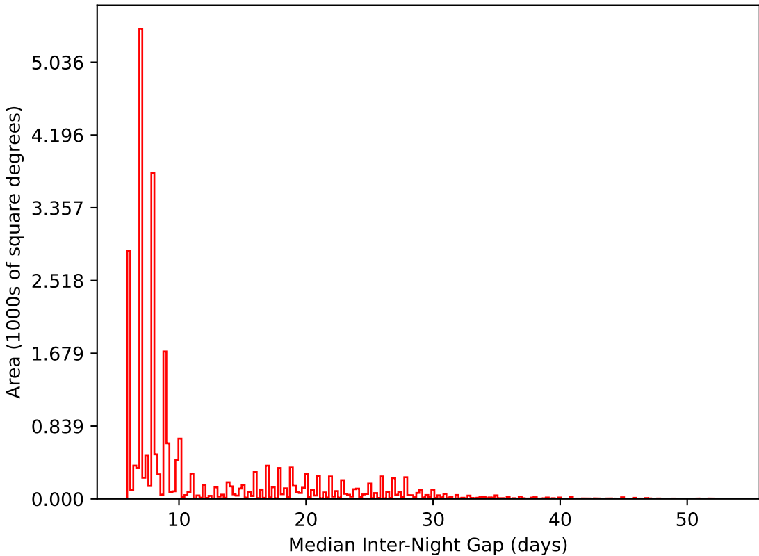
baseline_v2.0_10yrs All sky i band: Median Inter-Night Gap
