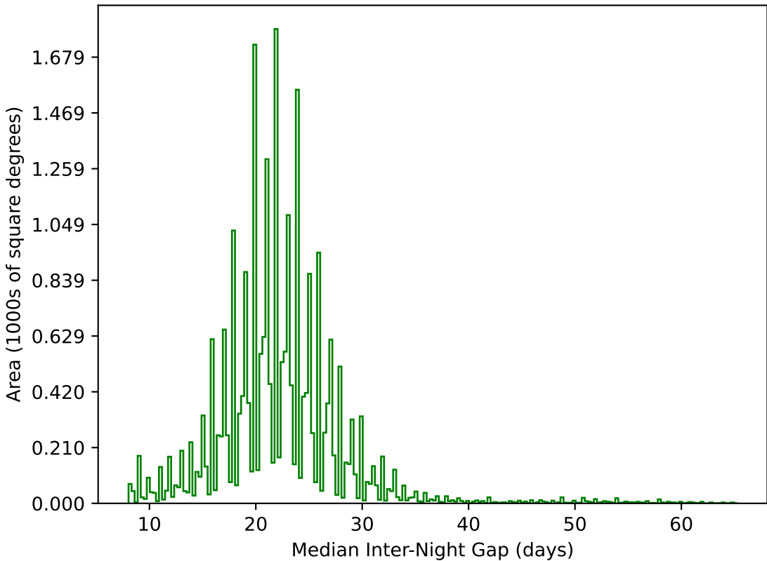
baseline_v2.0_10yrs All sky g band: Median Inter-Night Gap
