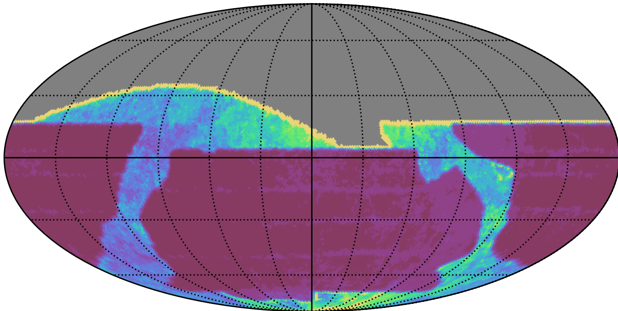
baseline_v2.0_10yrs All sky all bands: Median Inter-Night Gap
