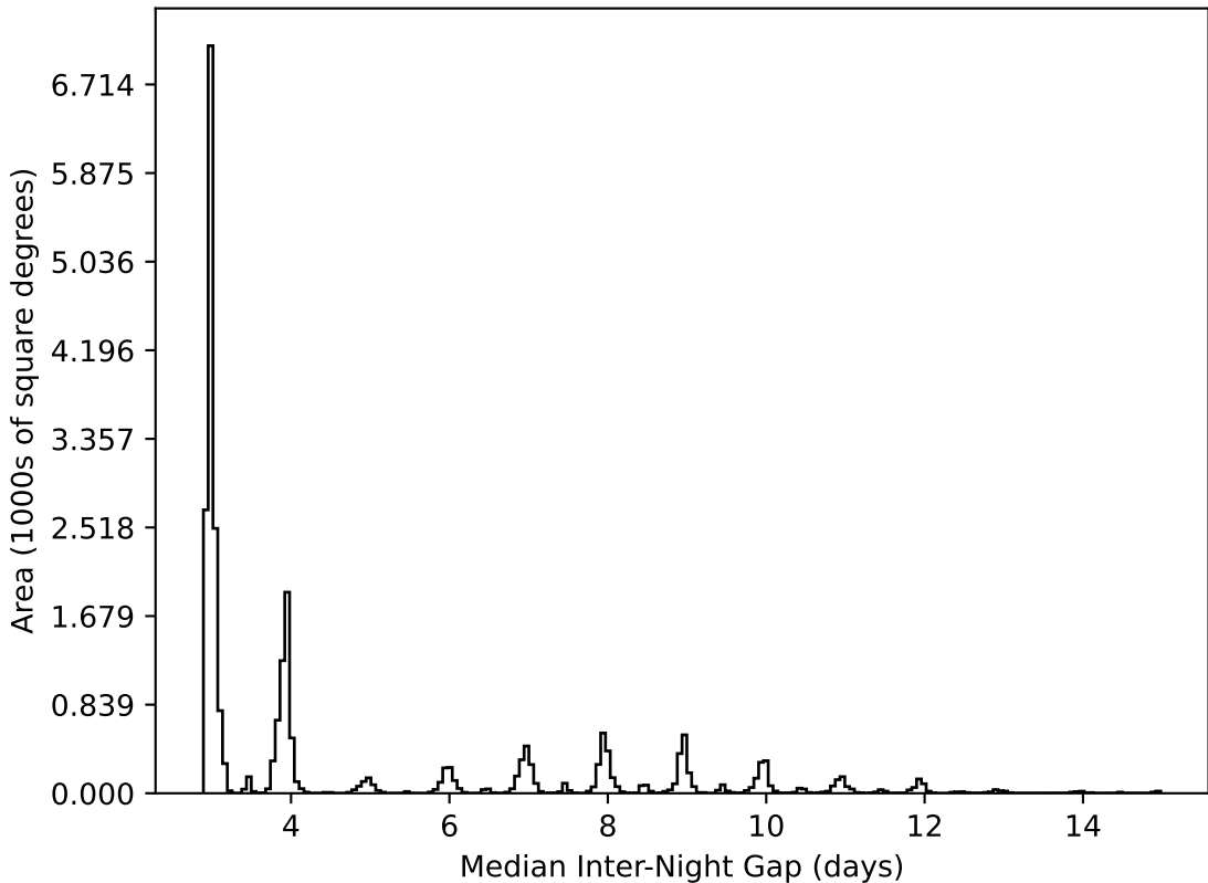
baseline_v2.0_10yrs All sky all bands: Median Inter-Night Gap
