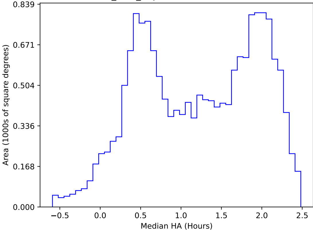
baseline_v2.0_10yrs WFD z band: Median HA
