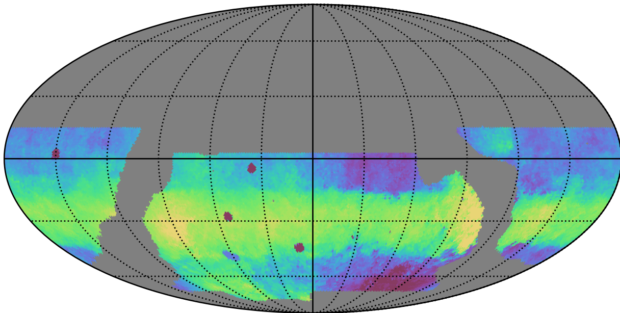
baseline_v2.0_10yrs WFD y band: Median HA
