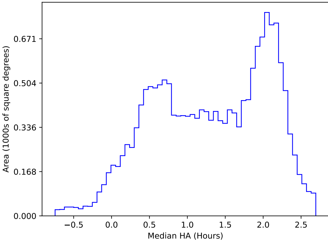
baseline_v2.0_10yrs WFD y band: Median HA
