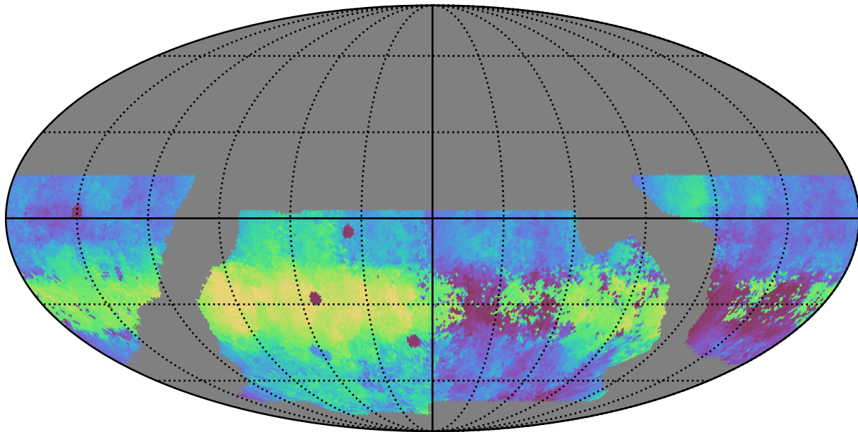
baseline_v2.0_10yrs WFD u band: Median HA
