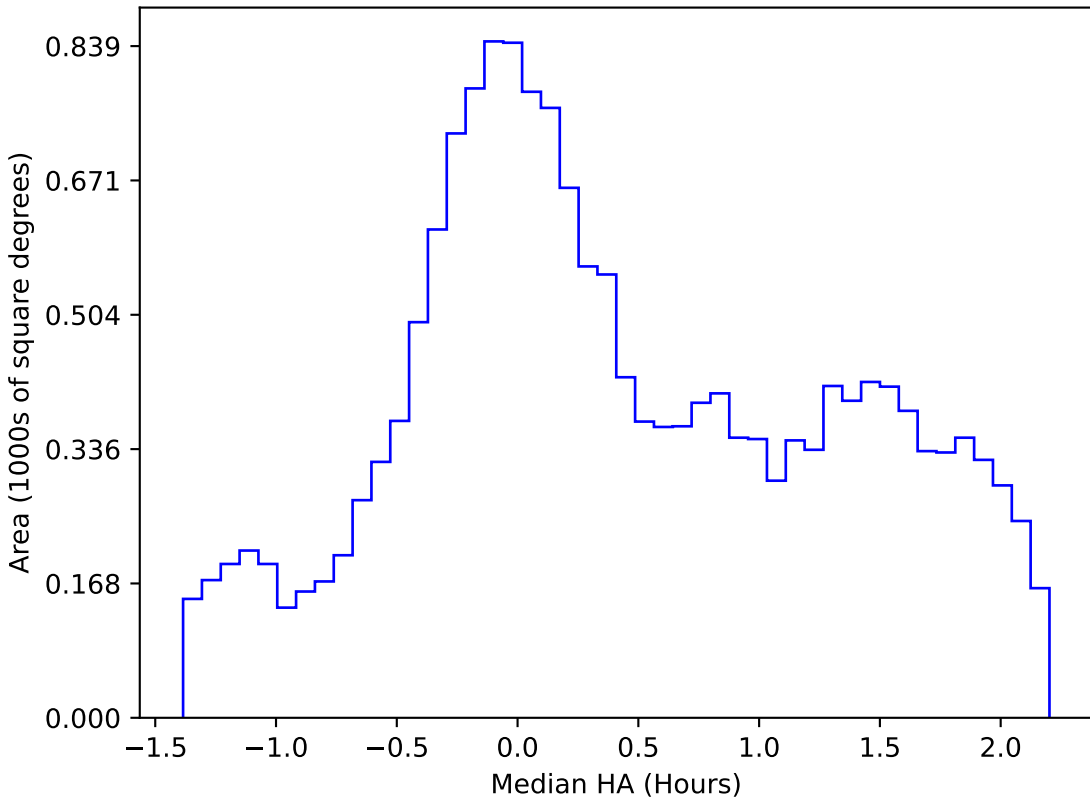
baseline_v2.0_10yrs WFD u band: Median HA
