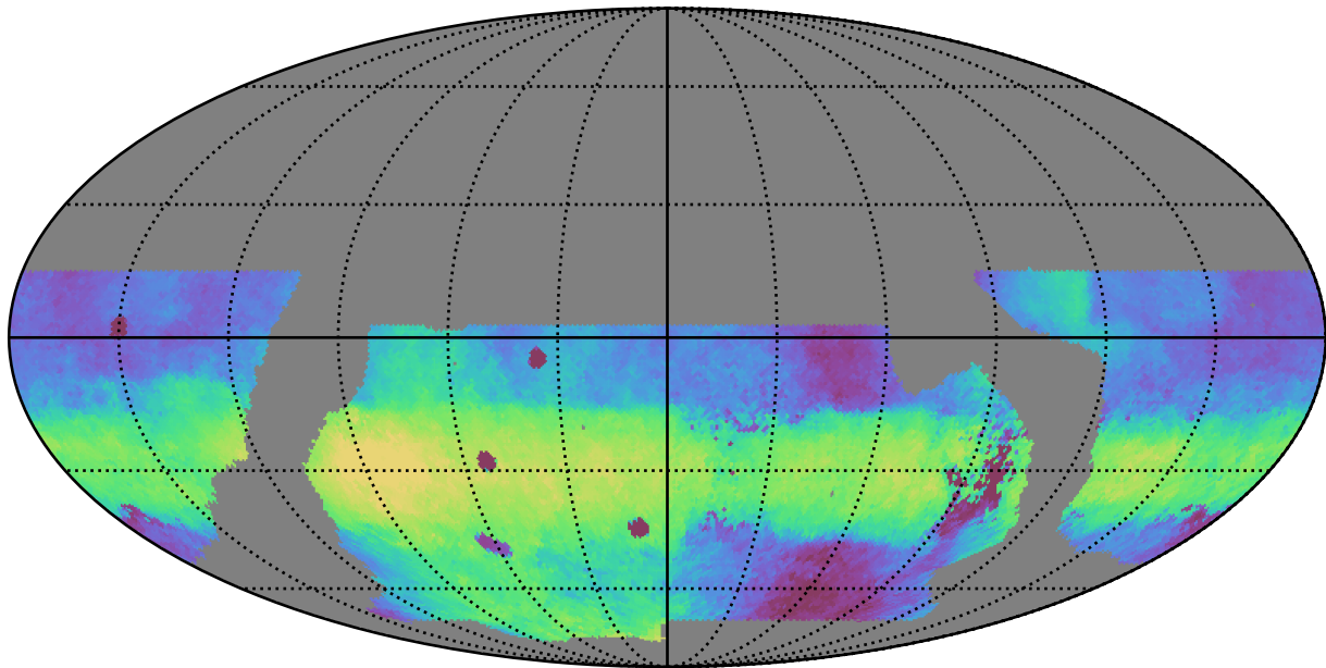
baseline_v2.0_10yrs WFD r band: Median HA
