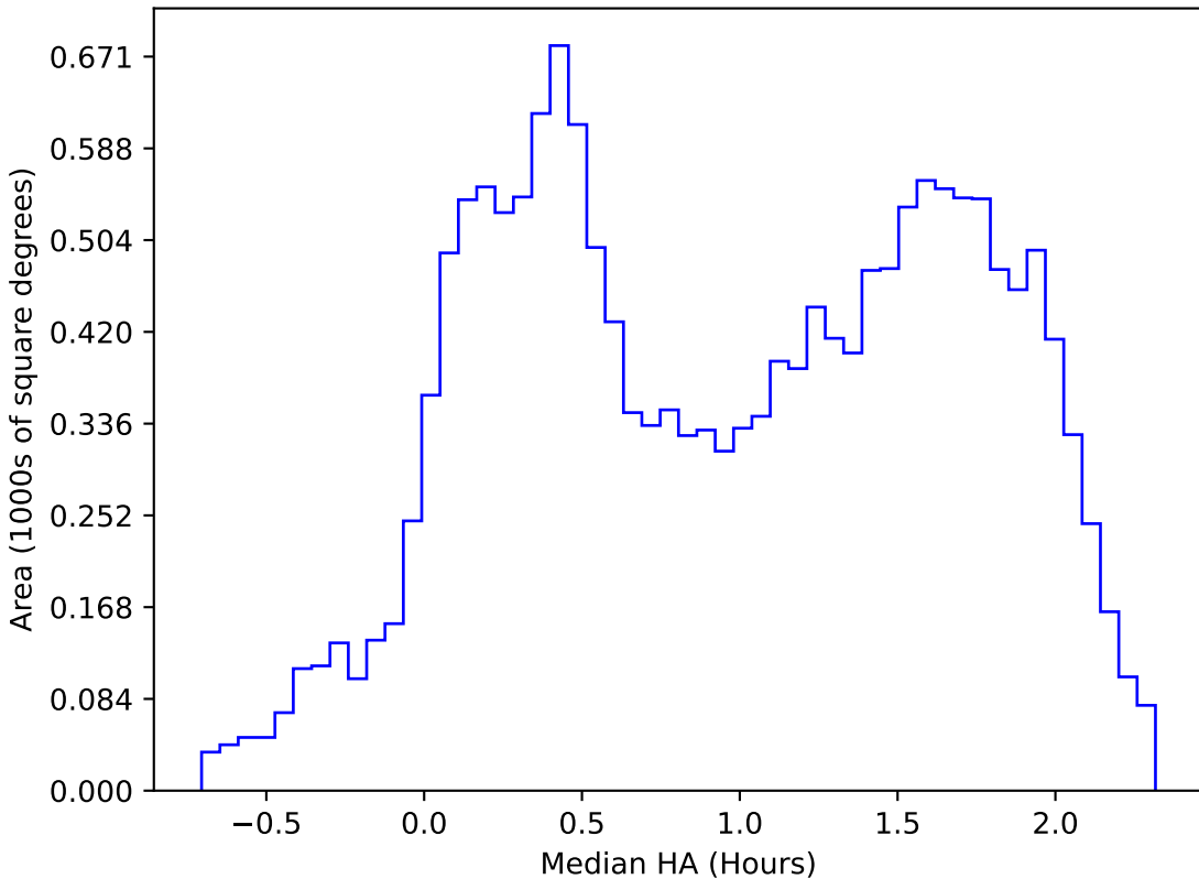
baseline_v2.0_10yrs WFD r band: Median HA
