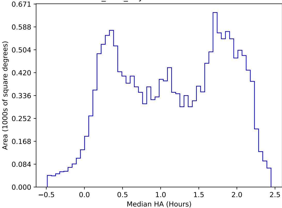
baseline_v2.0_10yrs WFD i band: Median HA
