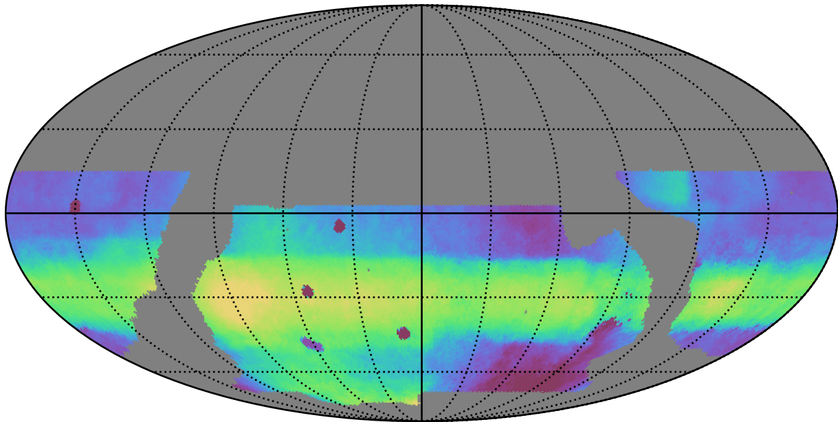
baseline_v2.0_10yrs WFD all bands: Median HA
