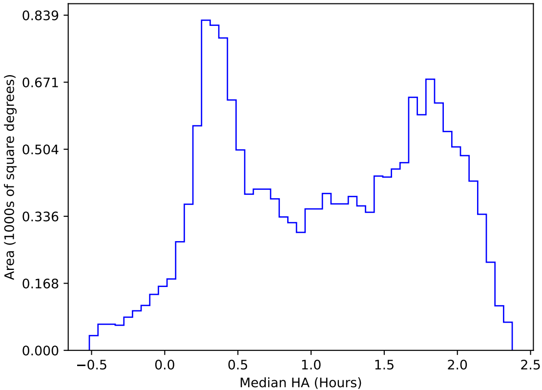
baseline_v2.0_10yrs WFD all bands: Median HA
