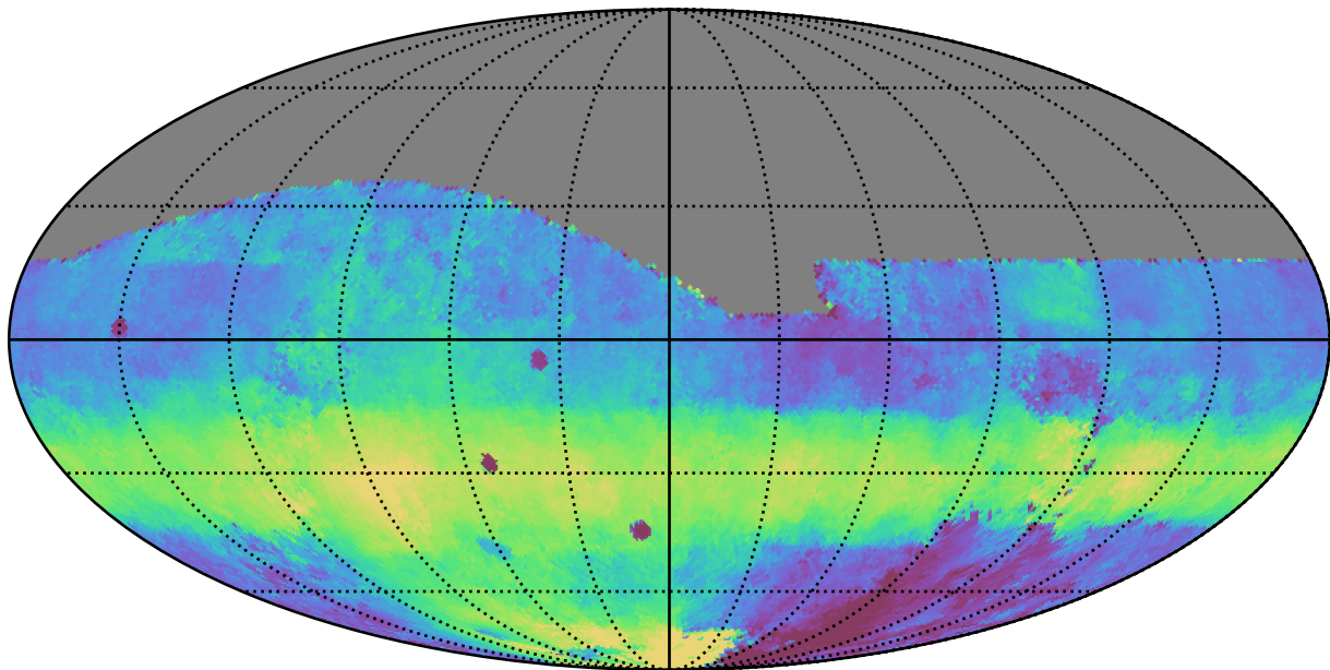
baseline_v2.0_10yrs All sky z band: Median HA
