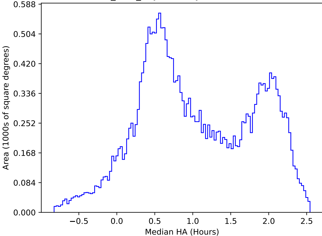
baseline_v2.0_10yrs All sky z band: Median HA
