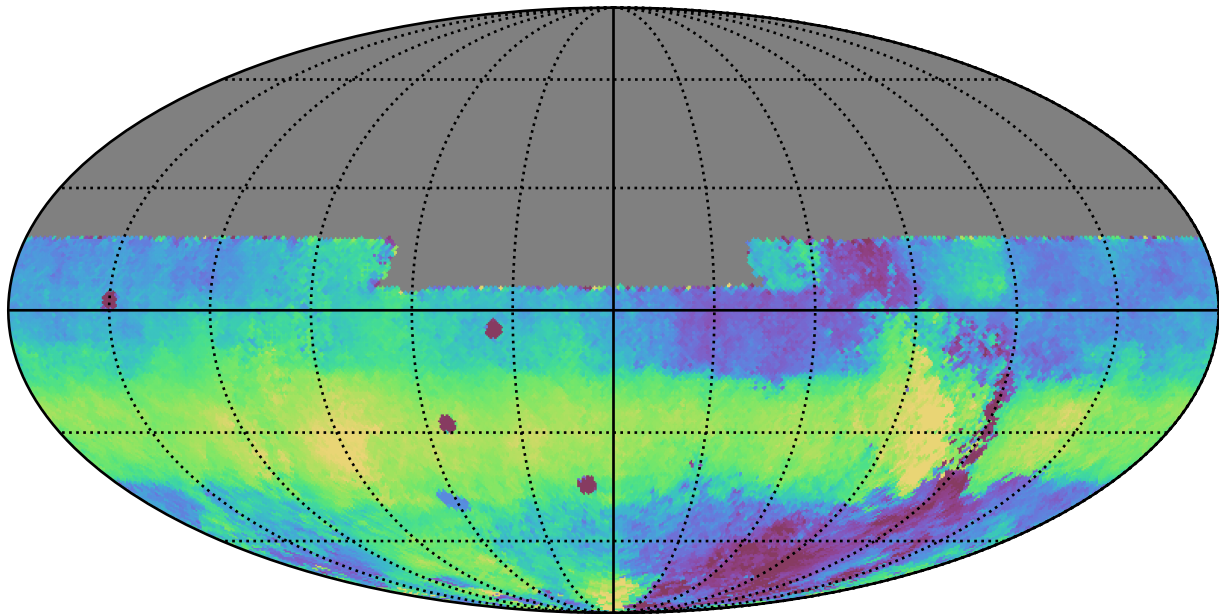
baseline_v2.0_10yrs All sky y band: Median HA
