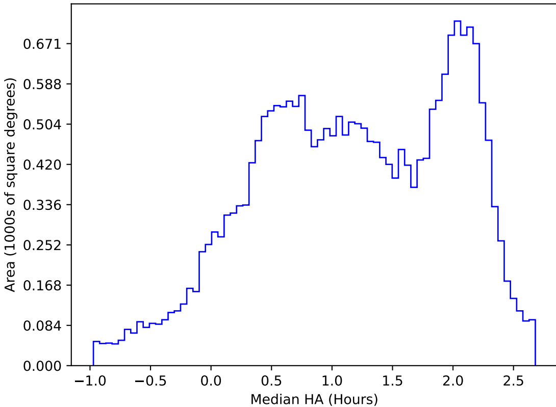
baseline_v2.0_10yrs All sky y band: Median HA
