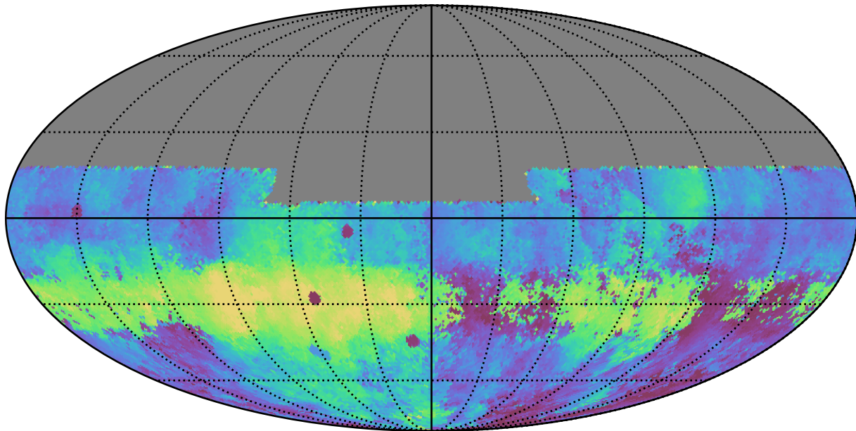
baseline_v2.0_10yrs All sky u band: Median HA
