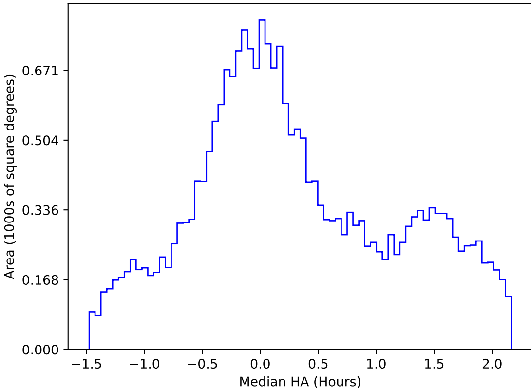
baseline_v2.0_10yrs All sky u band: Median HA
