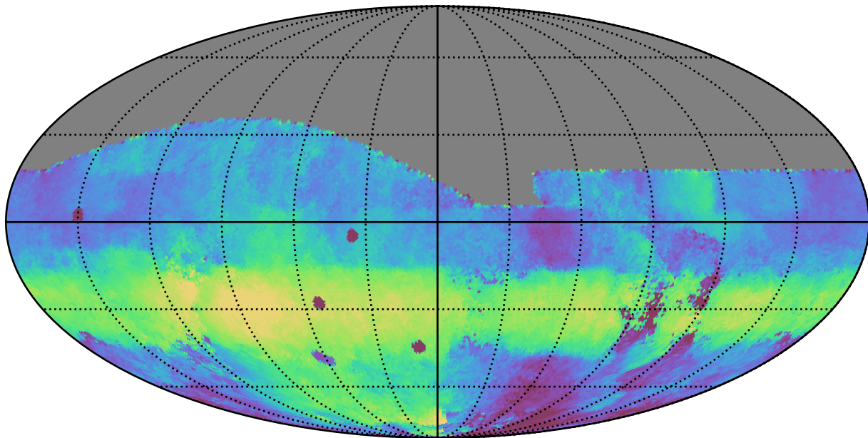
baseline_v2.0_10yrs All sky r band: Median HA
