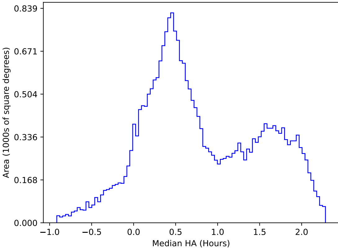
baseline_v2.0_10yrs All sky r band: Median HA
