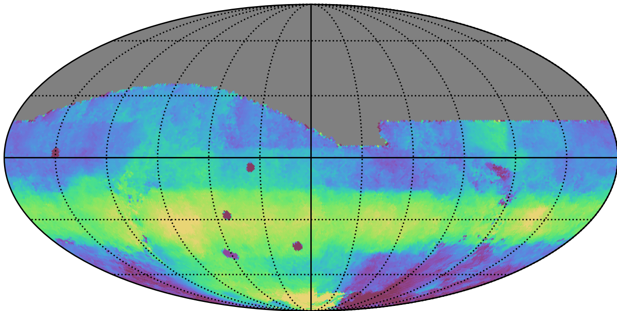
baseline_v2.0_10yrs All sky i band: Median HA
