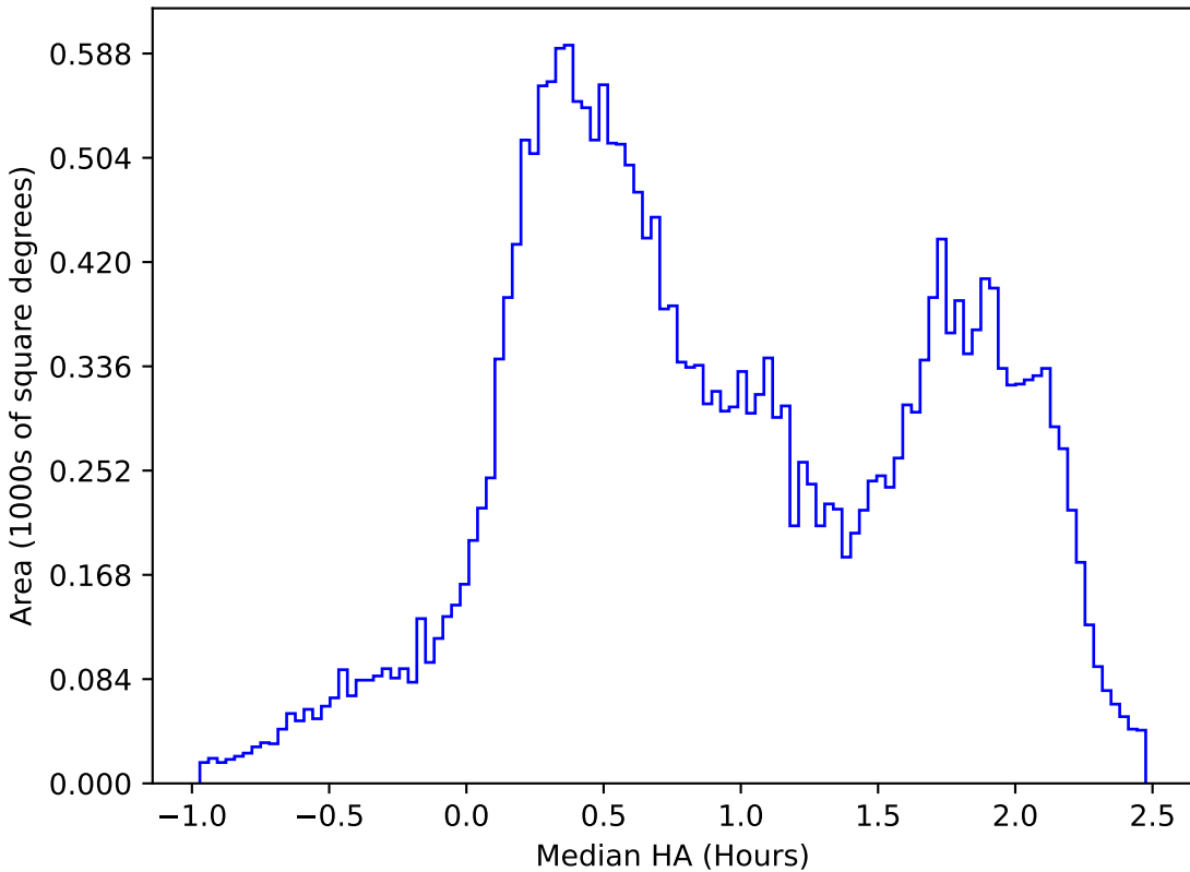
baseline_v2.0_10yrs All sky i band: Median HA
