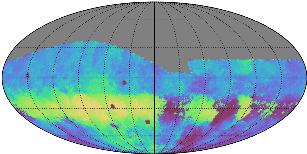
baseline_v2.0_10yrs All sky g band: Median HA
