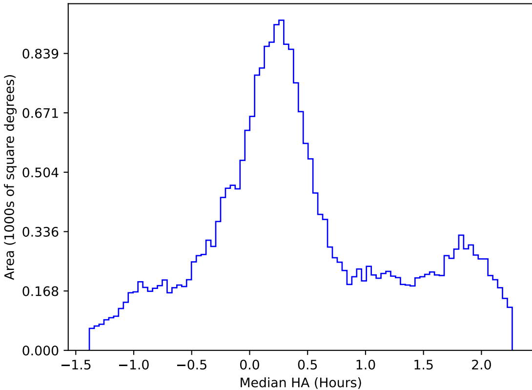
baseline_v2.0_10yrs All sky g band: Median HA
