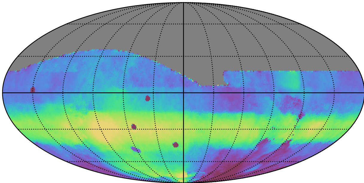
baseline_v2.0_10yrs All sky all bands: Median HA
