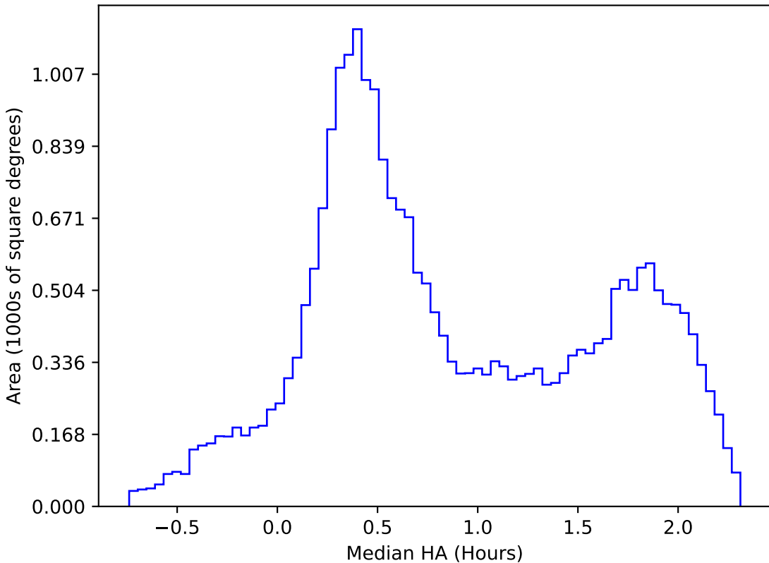
baseline_v2.0_10yrs All sky all bands: Median HA
