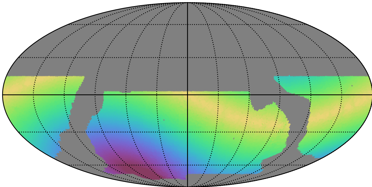
baseline_v2.0_10yrs WFD u band: Max solarElong
