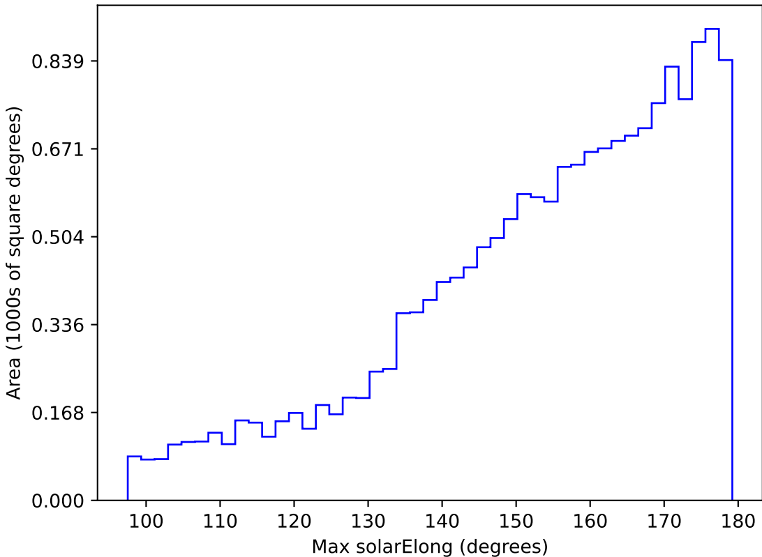
baseline_v2.0_10yrs WFD u band: Max solarElong
