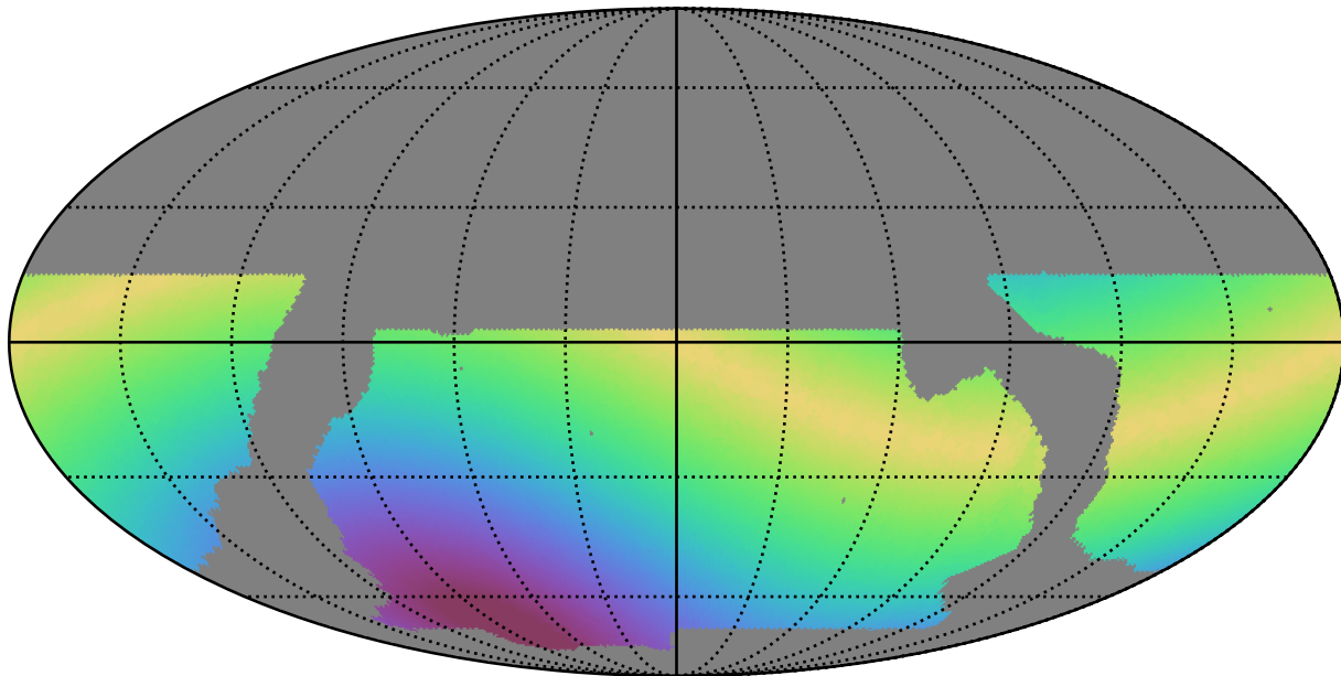
baseline_v2.0_10yrs WFD r band: Max solarElong
