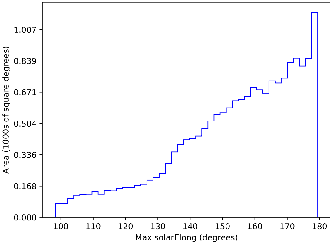
baseline_v2.0_10yrs WFD r band: Max solarElong
