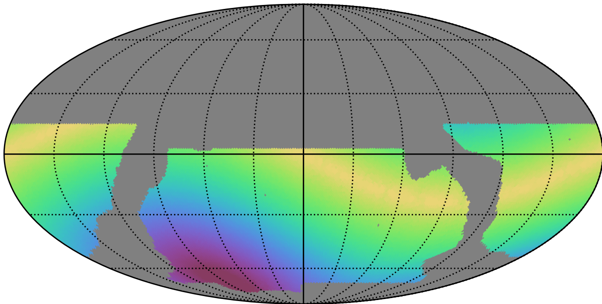
baseline_v2.0_10yrs WFD i band: Max solarElong
