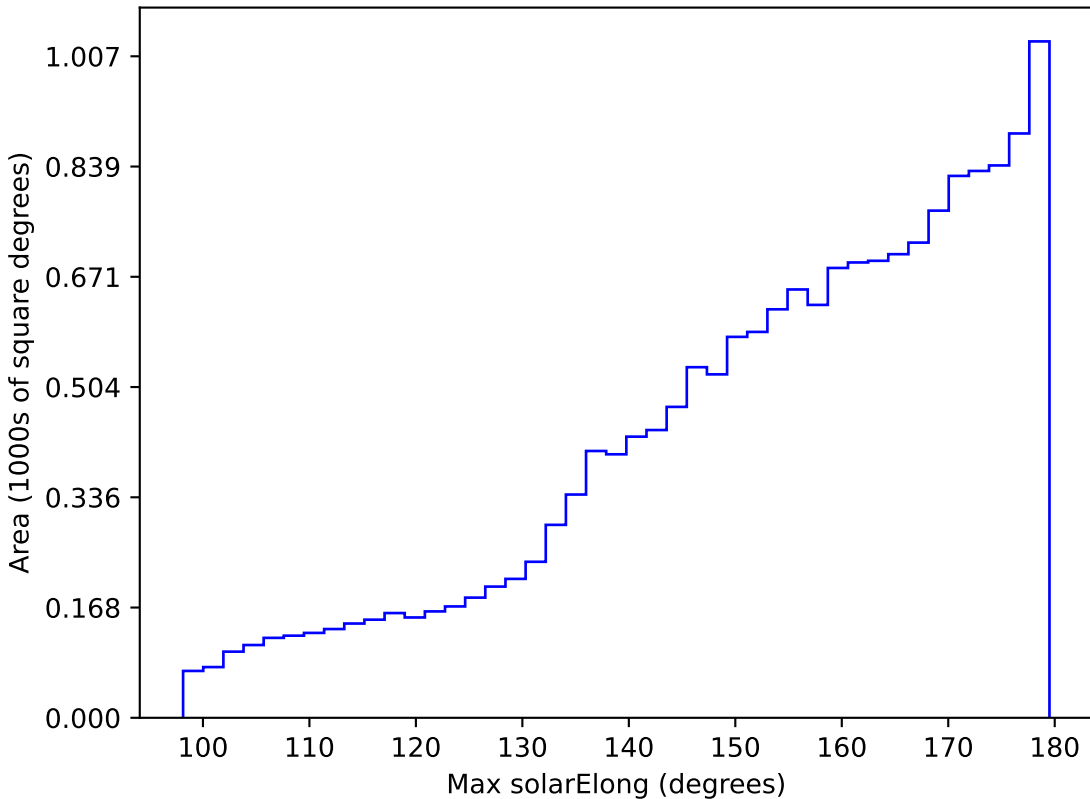
baseline_v2.0_10yrs WFD i band: Max solarElong
