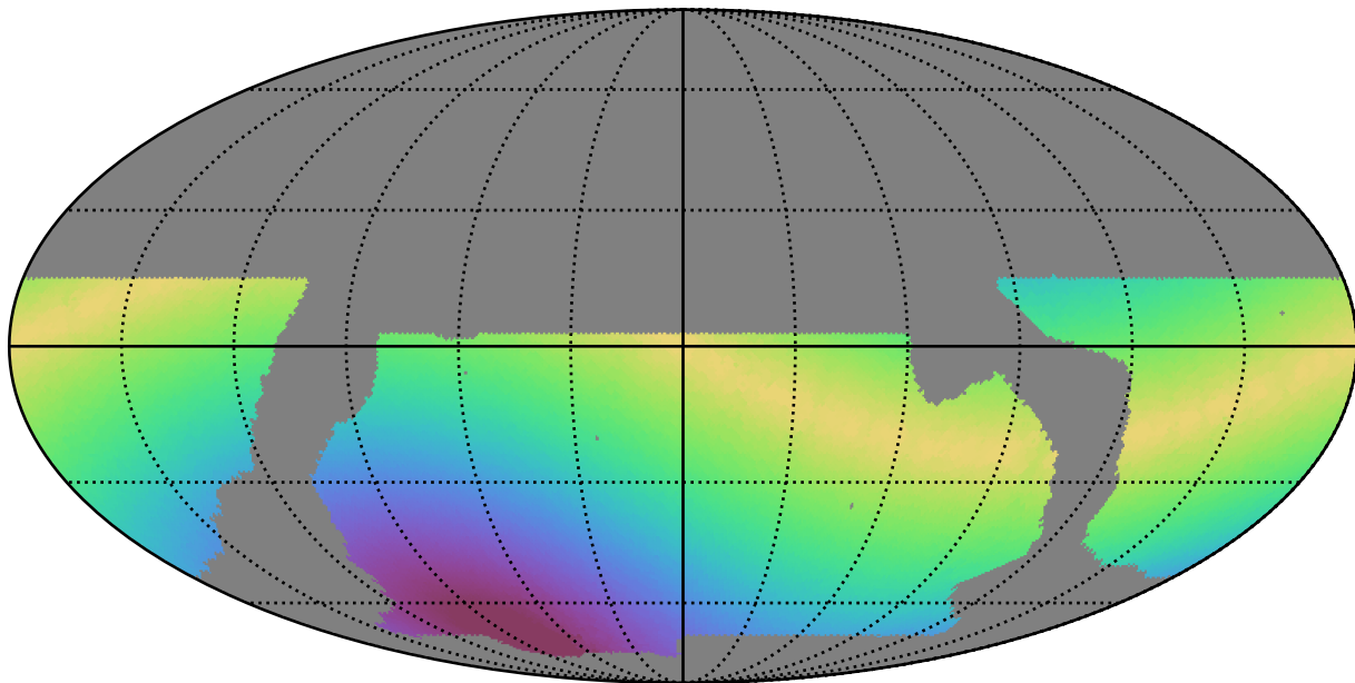
baseline_v2.0_10yrs WFD g band: Max solarElong
