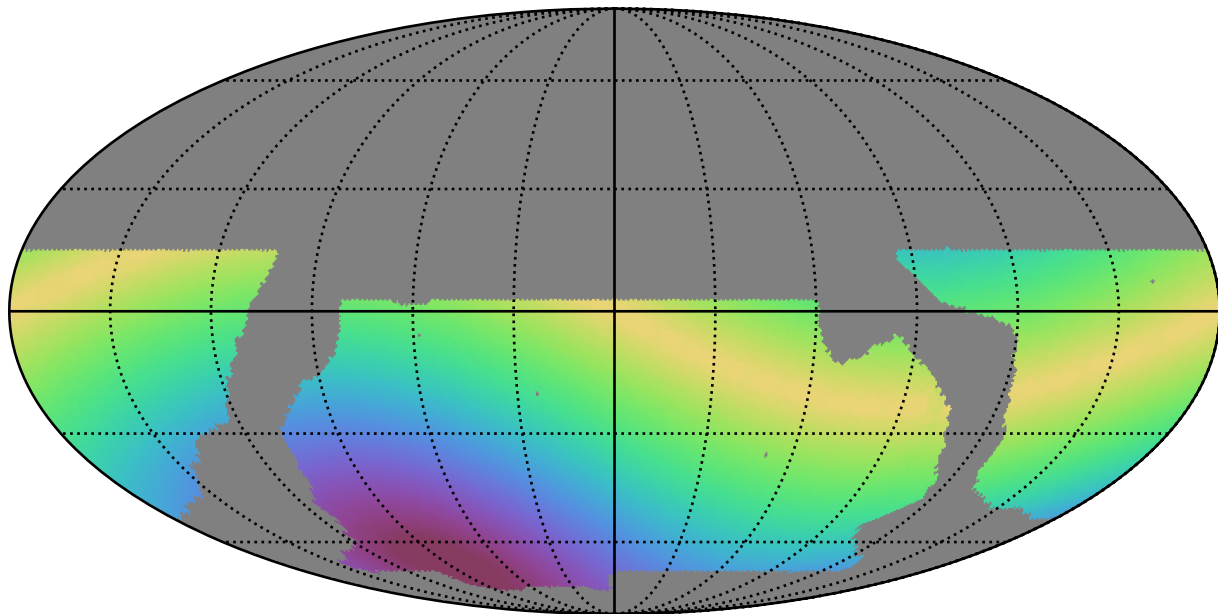
baseline_v2.0_10yrs WFD all bands: Max solarElong
