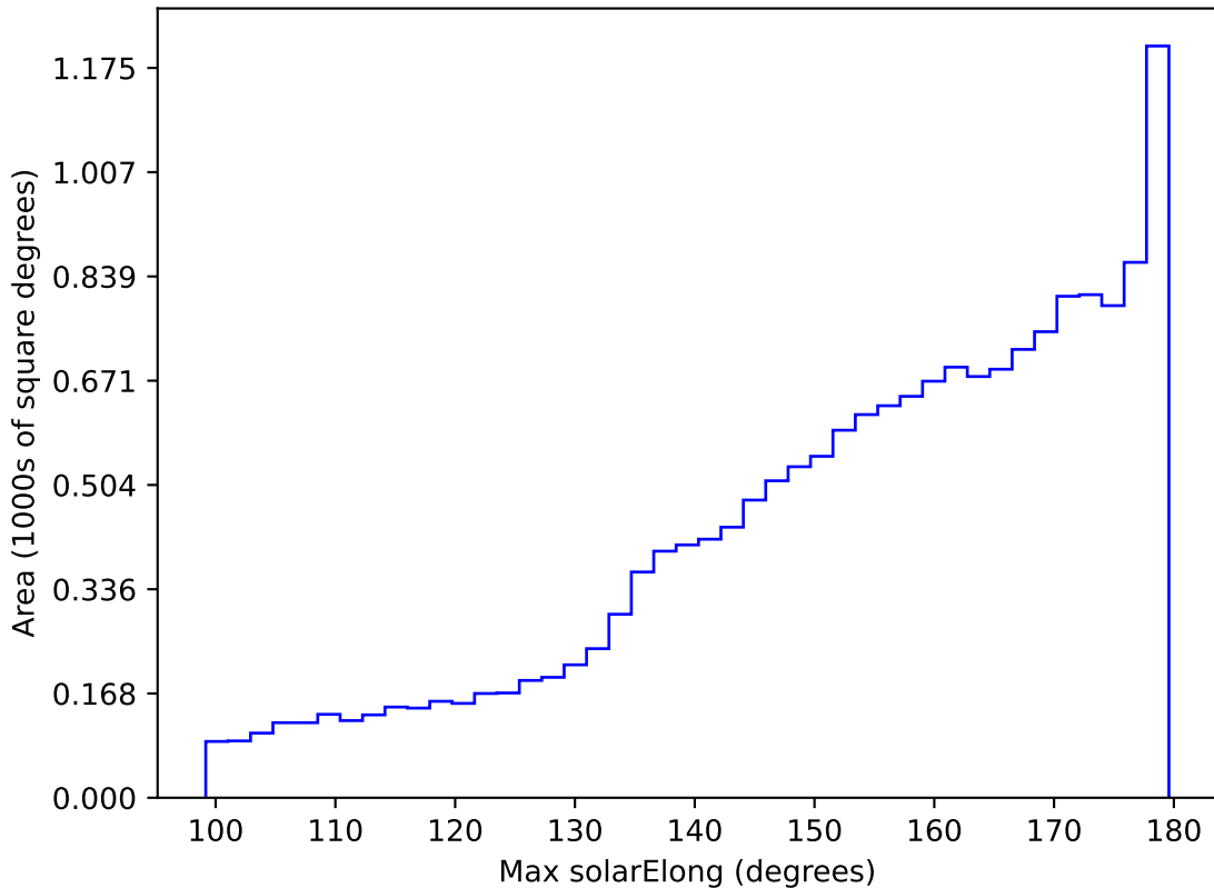
baseline_v2.0_10yrs WFD all bands: Max solarElong
