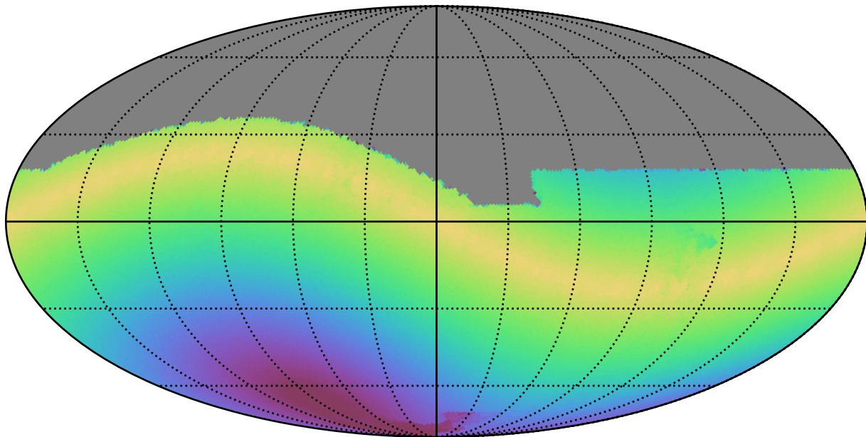
baseline_v2.0_10yrs All sky z band: Max solarElong
