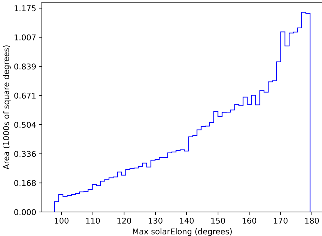
baseline_v2.0_10yrs All sky z band: Max solarElong
