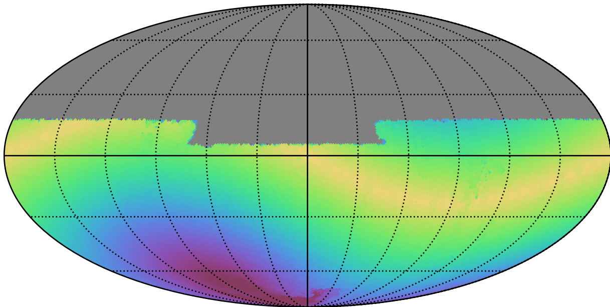
baseline_v2.0_10yrs All sky u band: Max solarElong
